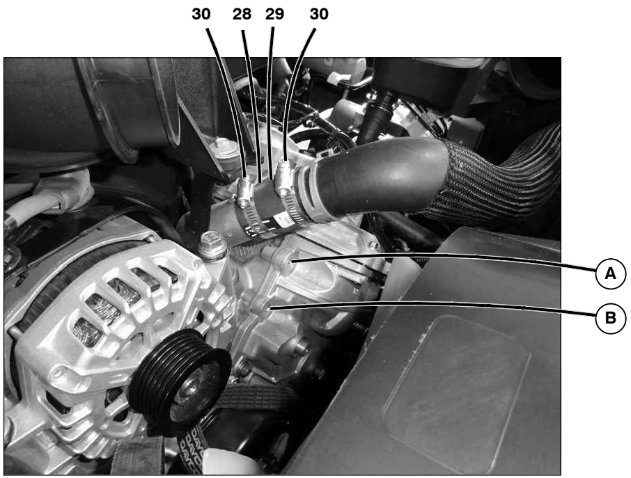
FIG. 5 BRACKET LOCATION RADIATOR HOSE SPLICE
